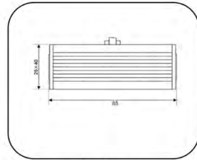
Dimension drawing
