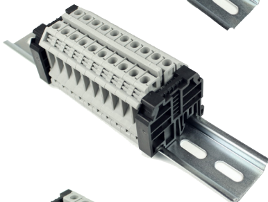
RAAK6NJ21-10 50 Amp, 300 Volt, with Jumpers
