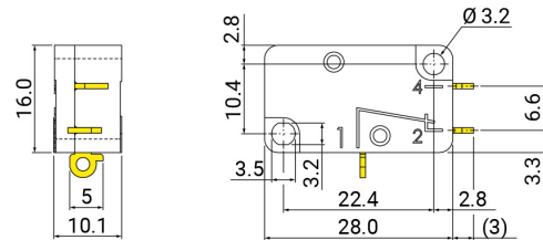
SOLDER TERMINALS
